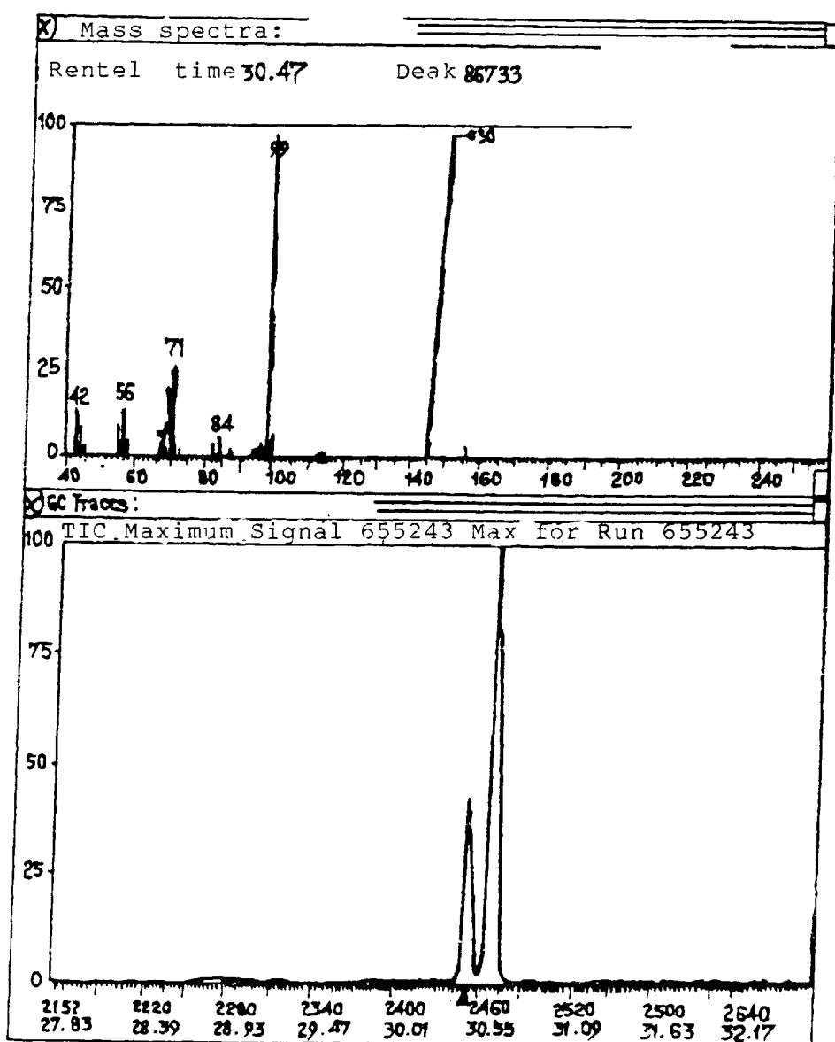
Mass spectra of 5-isobutyl-3-methyl-4,5-dihydro-2(3H) furanone.
